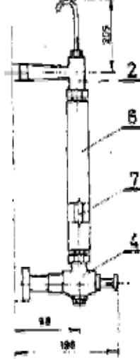
EXAMPLE OF EXECUTION B LEVEL GAUGE MARKING, LENGTH L = 1500 LEVEL GAUGE B 1500 – TYPE 3162
